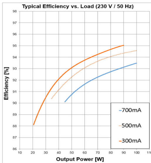
OTI DALI 100220-240700 D NFC IND L Typical Efficiency vs. Load (230 V 50 Hz)
