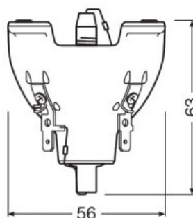
501949_Sirius HRI 330W XL
